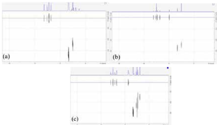
Fig. 8. ^1\text{H} DOSY NMR spectra of complexes in \text{DMSO-}d_6 : (a) 1 \text{ } ((\text{UO}_2)_2(\text{L}^1)_2) , C = 7.2 \text{ mM} ; (b) [2\text{-}4\text{DMF}] ((\text{UO}_2)_2(\text{L}^2)_2) , C = 6.1 \text{ mM} and (c) 3 \text{ } (\text{UO}_2\text{L}^3) , C = 2.1 \text{ mM} 28
