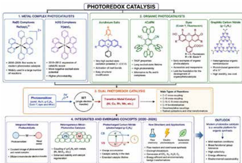
Fig. 7. Modern Photoredox Catalyst
