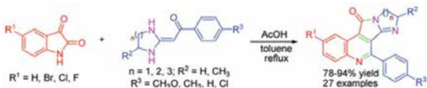
Fig. 11. The synthesis of substituted imidazopyrroloquinoline derivatives
