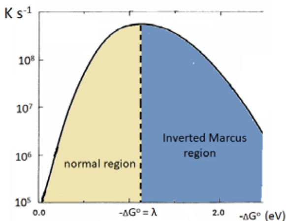
Fig. 8. Electron Transfer Rate in the Normal and Inverted Marcus Regions
